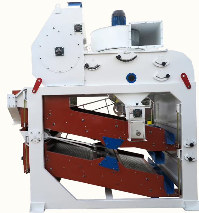
PCD – Paddy Cleaner Double deck (15 – 24 TPH)
