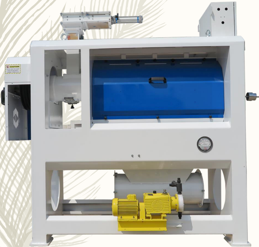
USP3 – Ultra Silky polisher (3 -4 TPH)
